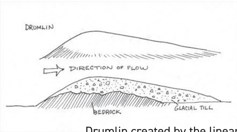
Drumlin created by the linear movement of Glaciers
